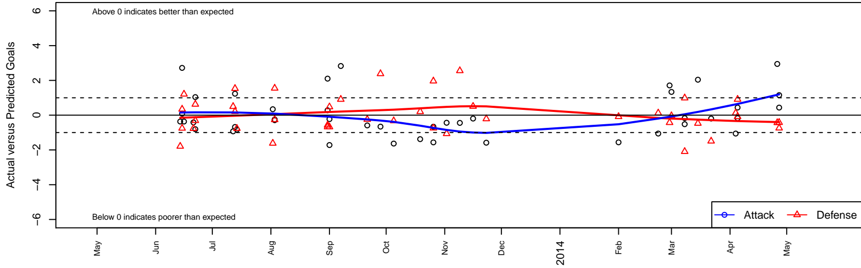
NW United MacKay G99 Dots are actual minus expected GF (blue circles) and GA (red triangles). Blue line is smoothed change in attack strength. Red is smoothed change in defense strength.
